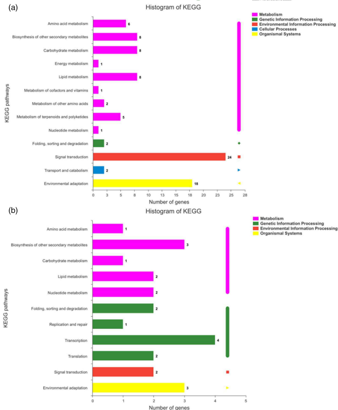
FIGURE 4 KEGG functional analysis and enrichment analysis were performed on the differentially expressed genes (DEGs). A histogram of KEGG function annotations was generated to compare the DEGs between AI&CK and PI&CK.
