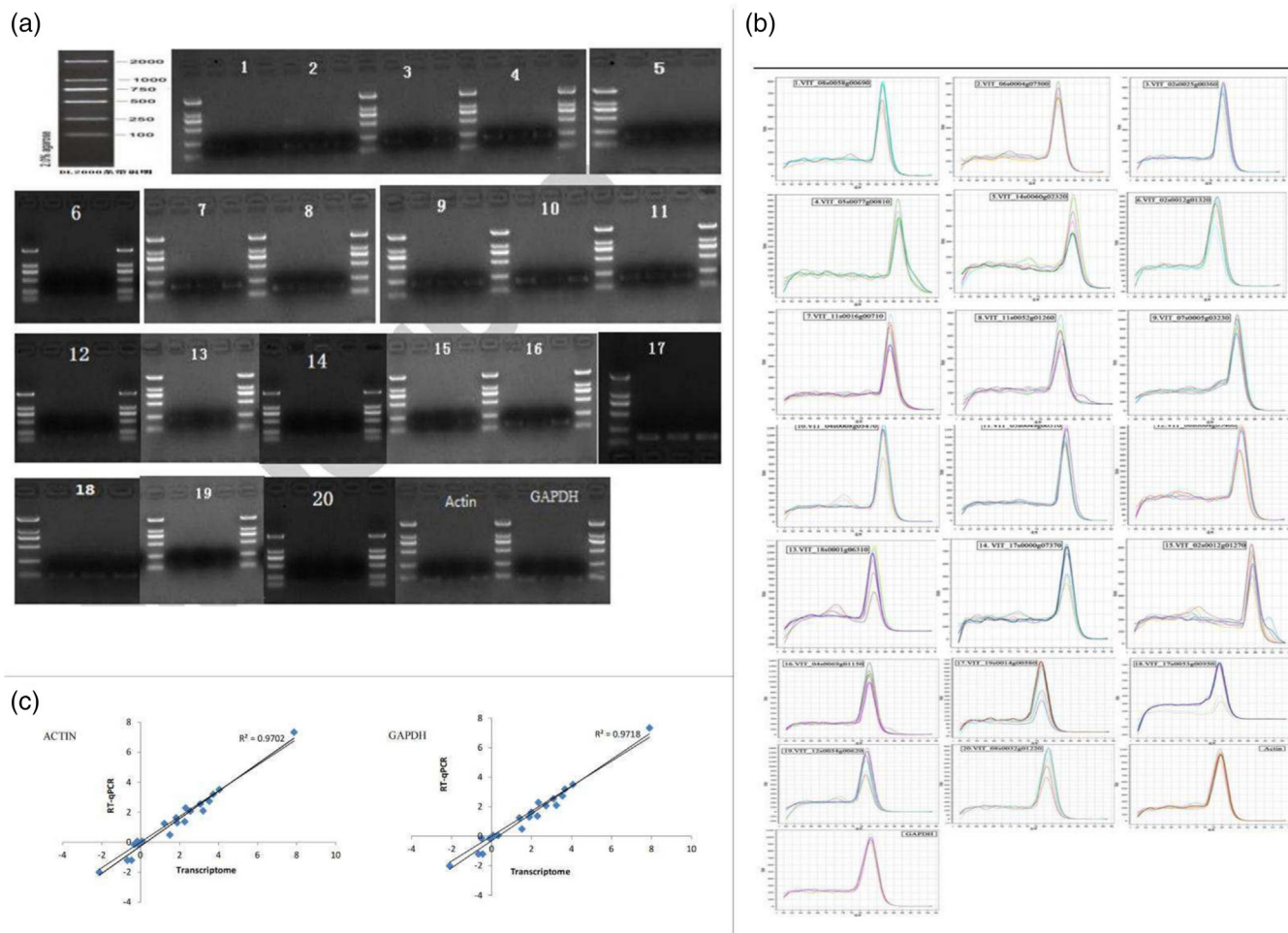
FIGURE 7 Validation map for RT-qPCR includes the following: (a) PCR amplification electrophoresis; (b) melting curves of 20 differential genes and internal reference genes; and (c) linear regression analysis of the RNA-seq and RT-qPCR data
