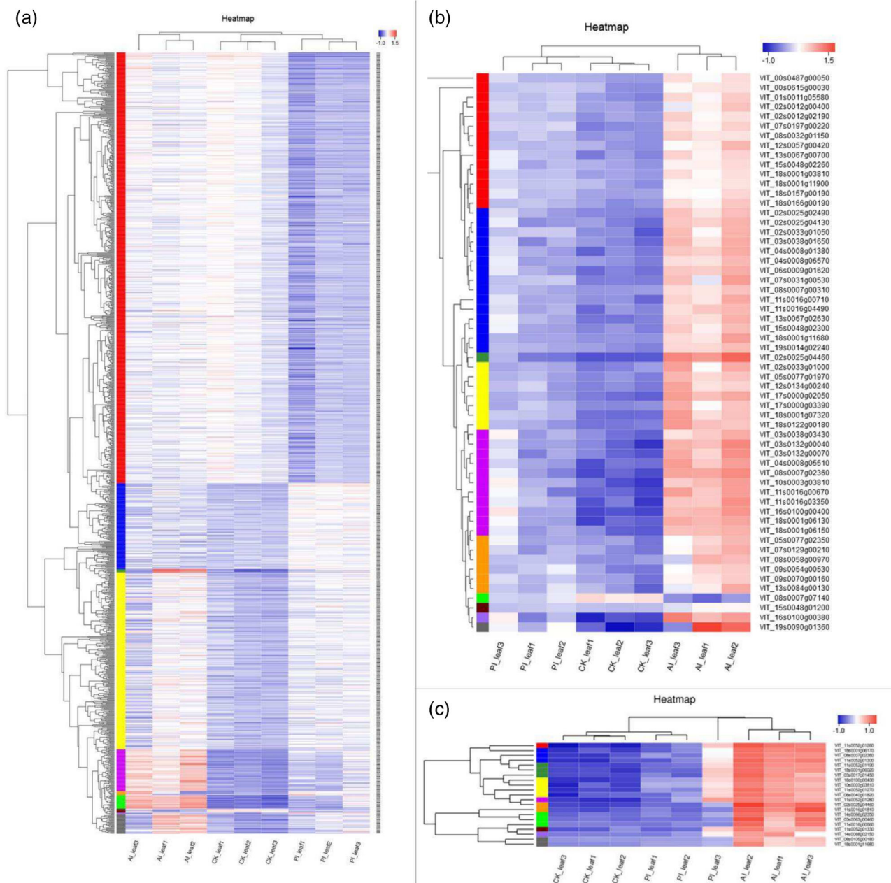
FIGURE 2 Cluster analysis was conducted on differentially expressed genes (DEGs) using the K-means algorithm. (a) Clustering pattern analysis of DEGs ( p adjust < .05). Note: Red represents upregulated genes, and blue represents downregulated genes. (b) Clustering pattern analysis of DEGs when Sum = 3. (c) |\text{Log}_2\text{FC}| \geq 5 pairs of screened DEGs cluster analysis with a difference of more than 5
