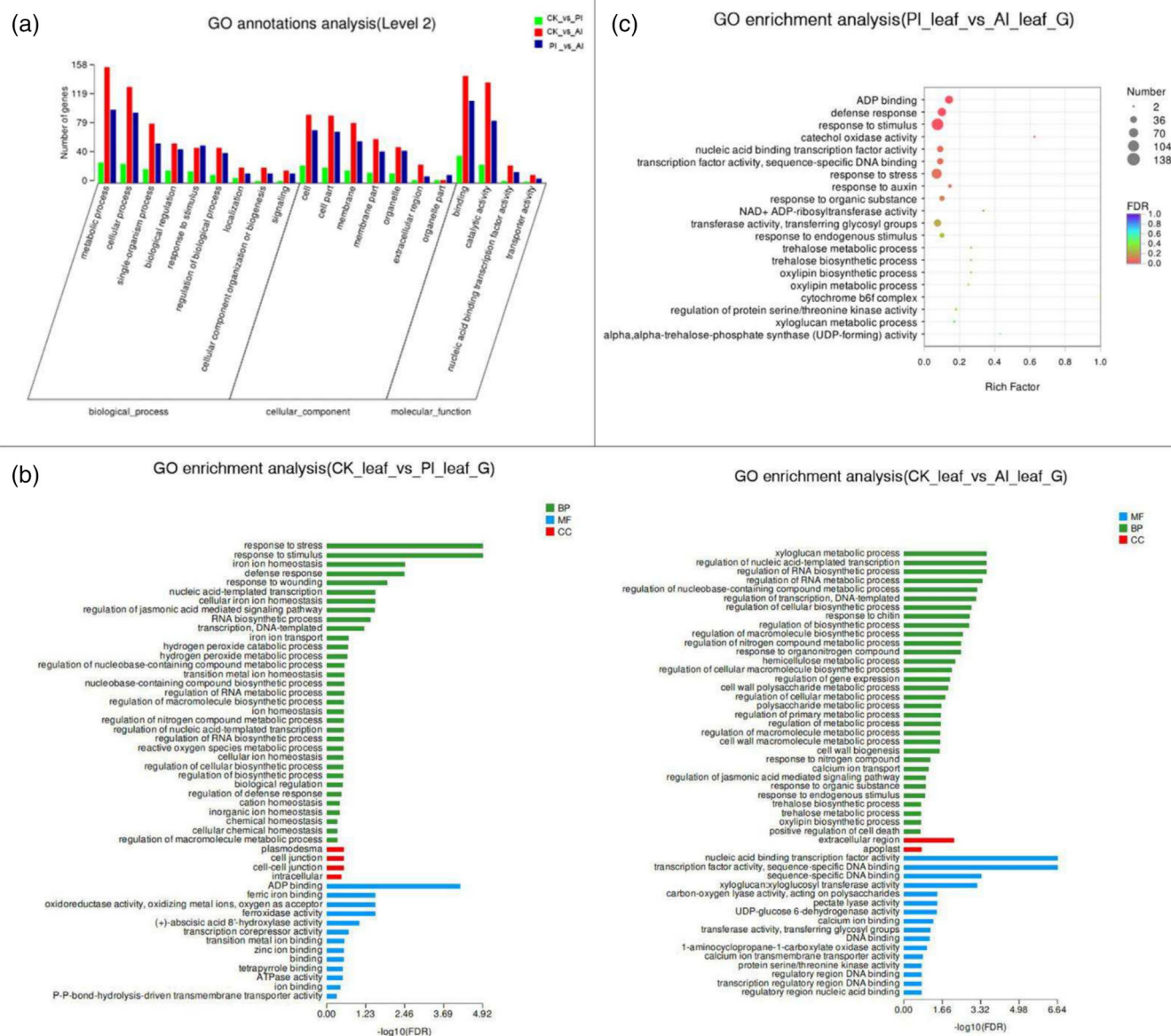
FIGURE 3 GO functional classification and metabolic pathway enrichment. (a) GO annotation of differentially expressed genes (DEGs) in various treatments ( |\log_2FC| \geq 2 ). Note: The x axis represents the functional categories of GO, and the y axis represents the number of genes associated with each function. (b) GO enrichment analysis of DEGs between the PI and CK treatments and the AI and CK treatments. (c) GO enrichment analysis of DEGs between the AI and PI treatments
