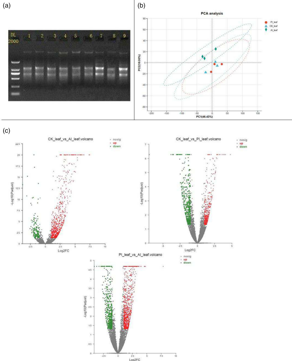
FIGURE 1 RNA quality analysis on nine “Cabernet Sauvignon” grape leaf samples and analysis of differentially expressed genes (DEGs) among the three treatments. (a) RNA quality detection showing clear and complete bands for all nine samples. (b) PCA analysis was performed to examine the differential genes among the three treatments. (c) Volcano maps were created to visualize the DEGs across the different treatments.
