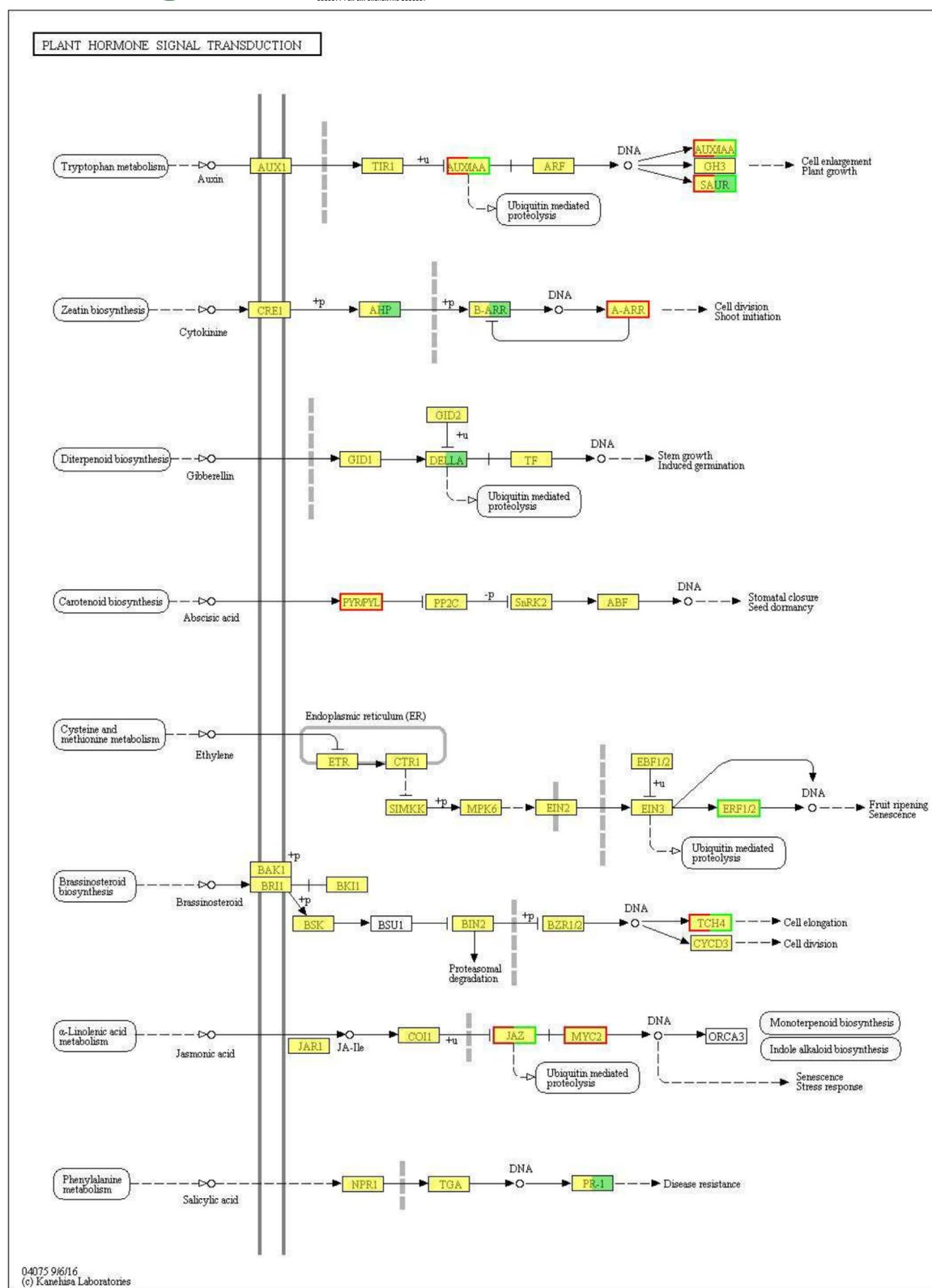
FIGURE 6 Compared with the CK treatment, the signal pathway map of DEGs in the AI treatment was significantly localized. Map 04075 is the plant hormone signal transfer pathway, and homologous genes such as JAZ and MYC2 have been annotated. Map 04626 is the interaction metabolic pathway of plant pathogens, which is mainly mapped to the expression of defense genes related to \text{Ca}^{2+} and allergic reactions. Map 04016 is the MAPK signaling pathway, in which the phosphorylation of MAPK kinases causes the stress response of “Cabernet Sauvignon.” Note: “ ” represents known genes/transcripts, “ ” represents upregulated genes, “ ” represents downregulated genes, “ ” represents up + downregulated genes, “ ” represents new genes/transcripts, and “ ” represents known + new genes/transcripts.
